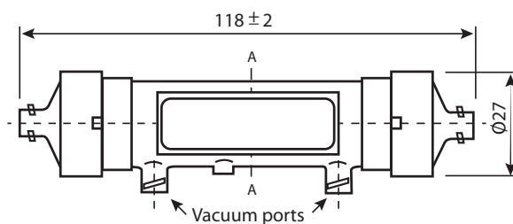
Figure 1: Dimensions in mm
